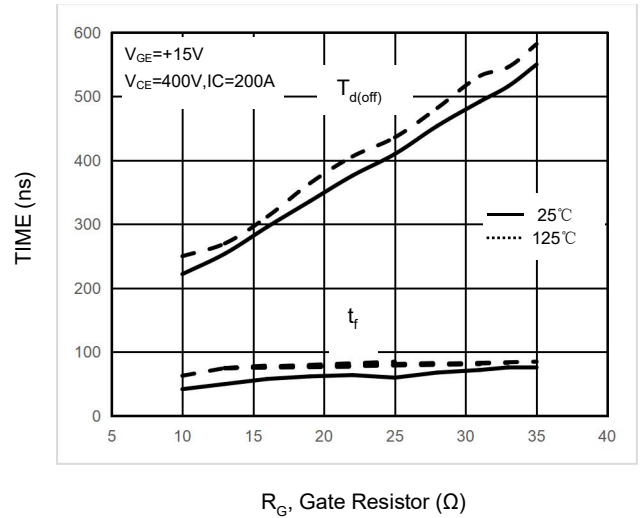
Figure 28. Typical Switching Time T_{doff} vs. R_G
