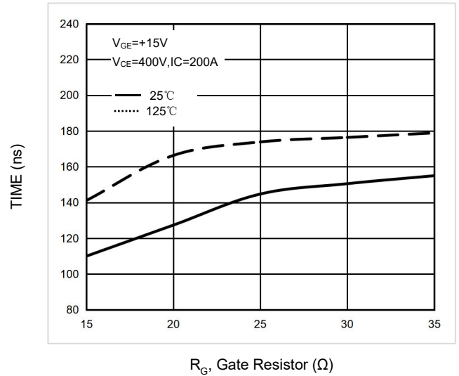
Figure 30. Typical Reverse Recovery Time vs. R_G
