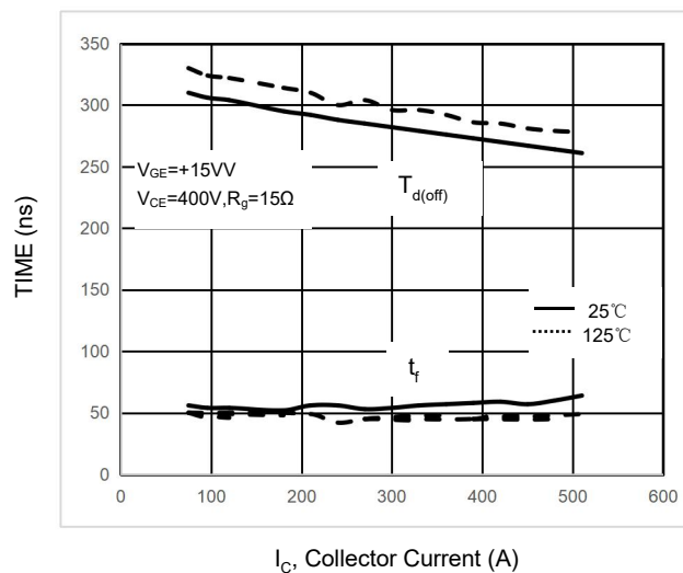
Figure 26. Typical Switching Time T_{doff} vs. I_C
