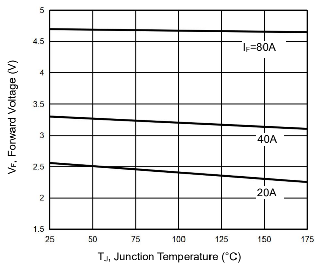
Figure 8 V_F vs. Temperature
