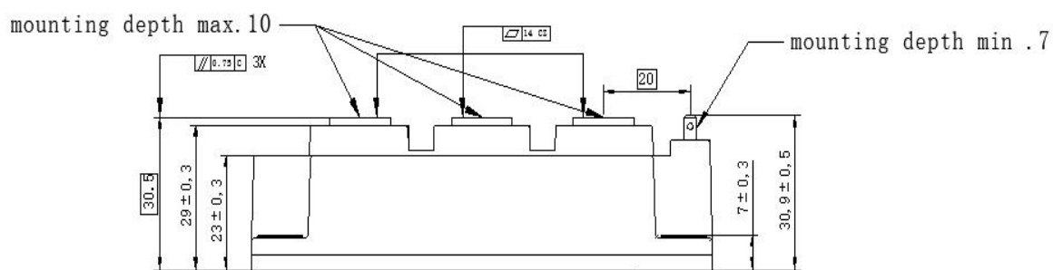
SIDE VIEW
