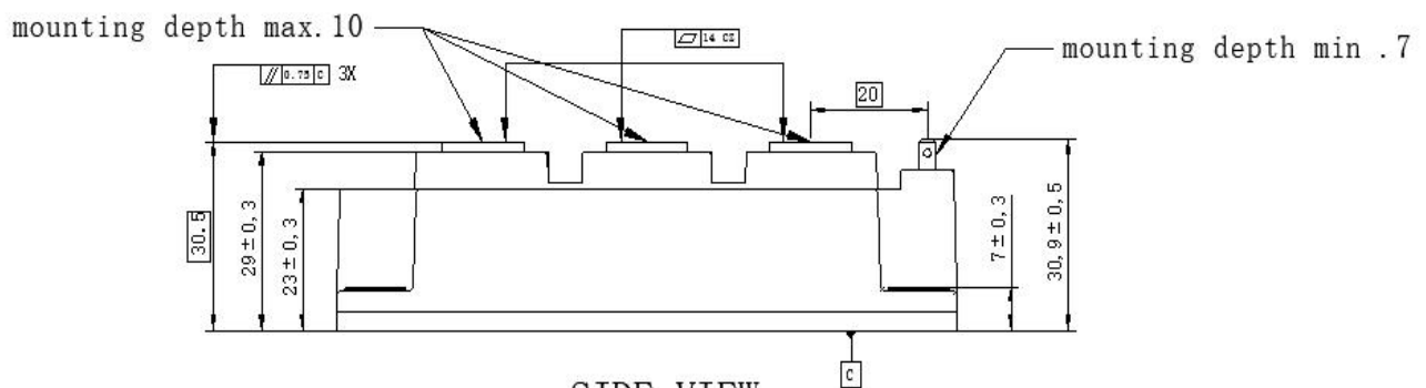
SIDE VIEW
