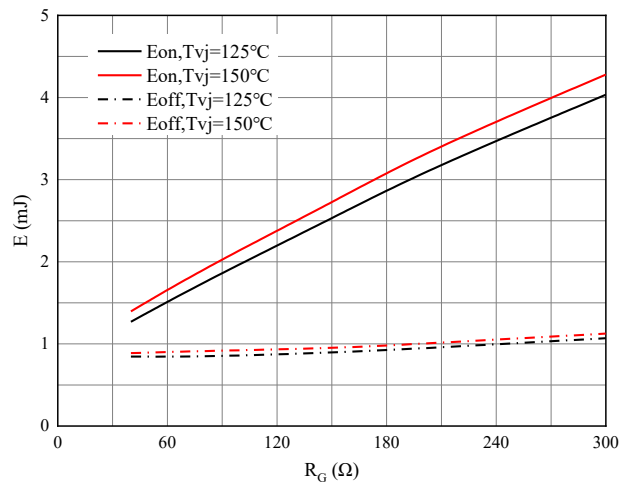
Fig 6. Switching losses of IGBT
