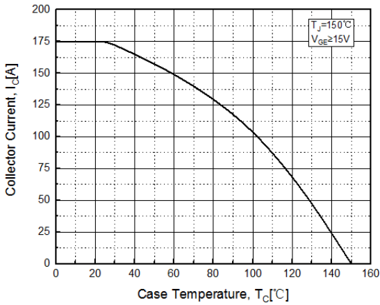
Fig. 7. Rate Current vs. T_C
