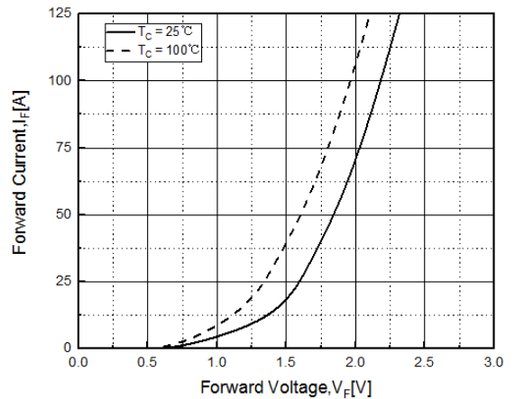
Fig. 10. Forward Characteristics
