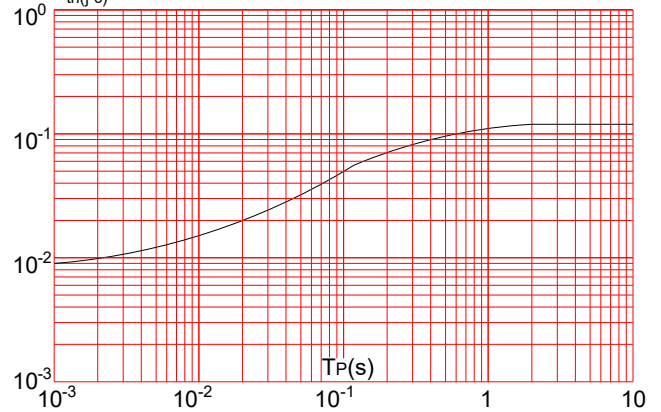
FIG.4: Maximum transient thermal impedance R_{th(j-c)} (K/W) Junction-to-case(per diode)
