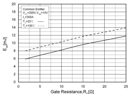
Fig. 5. Turn-on Characteristics vs. R_G
