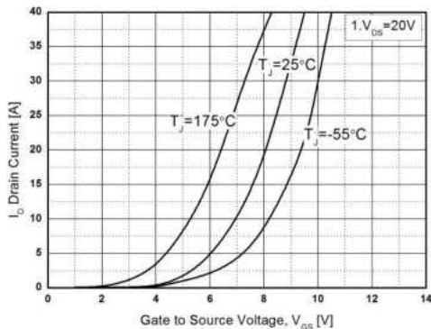
Fig. 5. Transfer Characteristics
