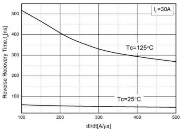
Fig. 3. Typical Reverse Recovery Time vs. di/dt
