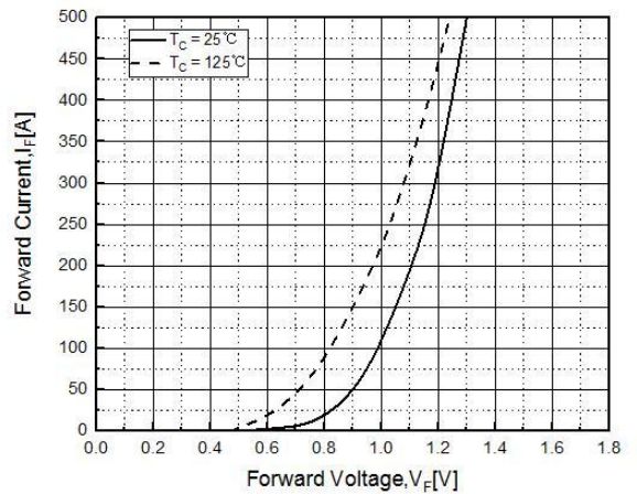
Fig. 10. Forward Characteristics
